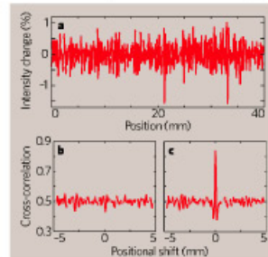
Figure 1 | Comparing document fingerprints. a, The fluctuation in diffuse intensity at one photodetector as a focused laser beam is scanned across a 40-mm length of white paper. b, Digital cross-correlation between two scans from different sheets of paper. c, Digital cross-correlation between two scans from the same sheet of paper.
